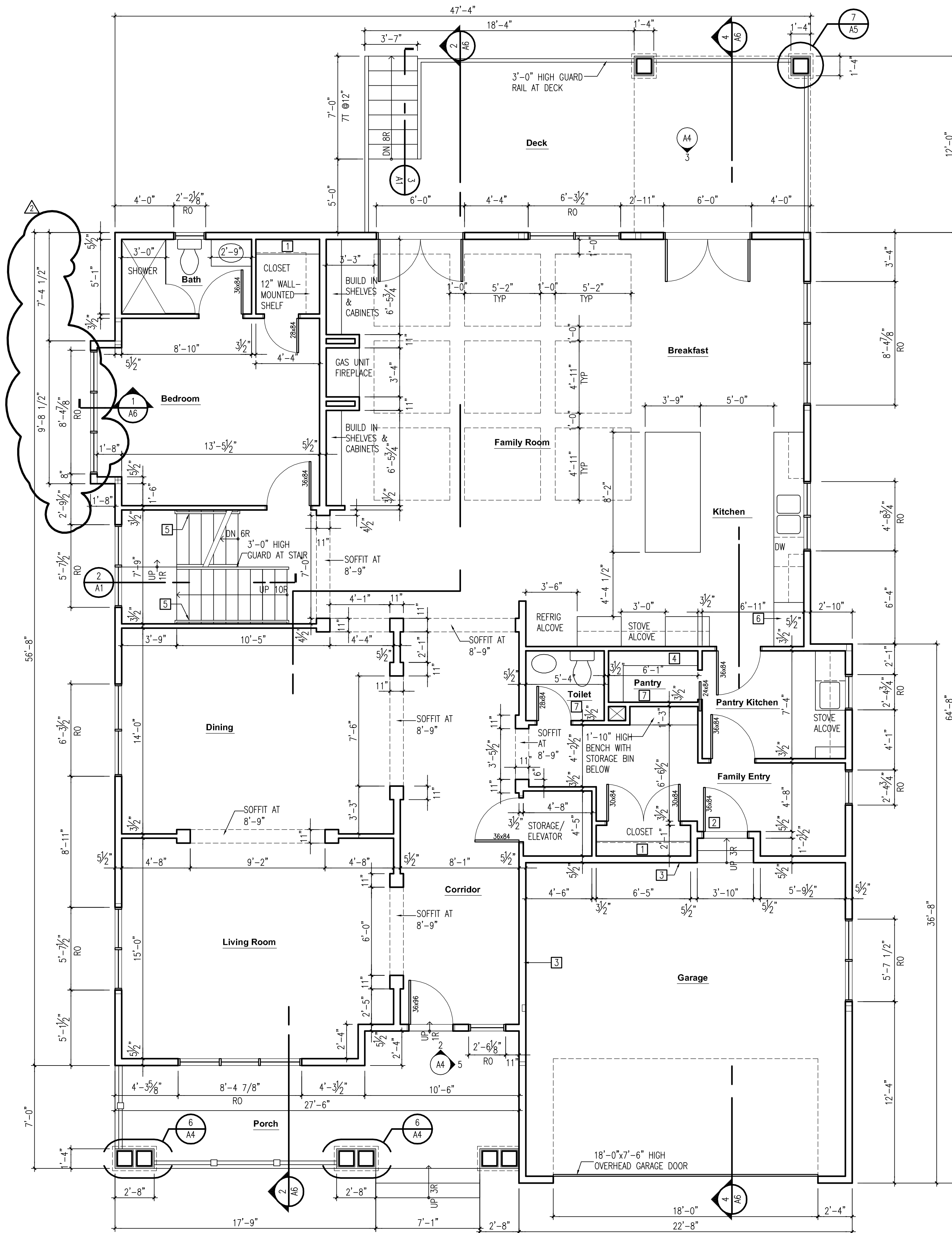
1 FIRST FLOOR PLAN SCALE: 1/4"=1'-0" plan NORTH
