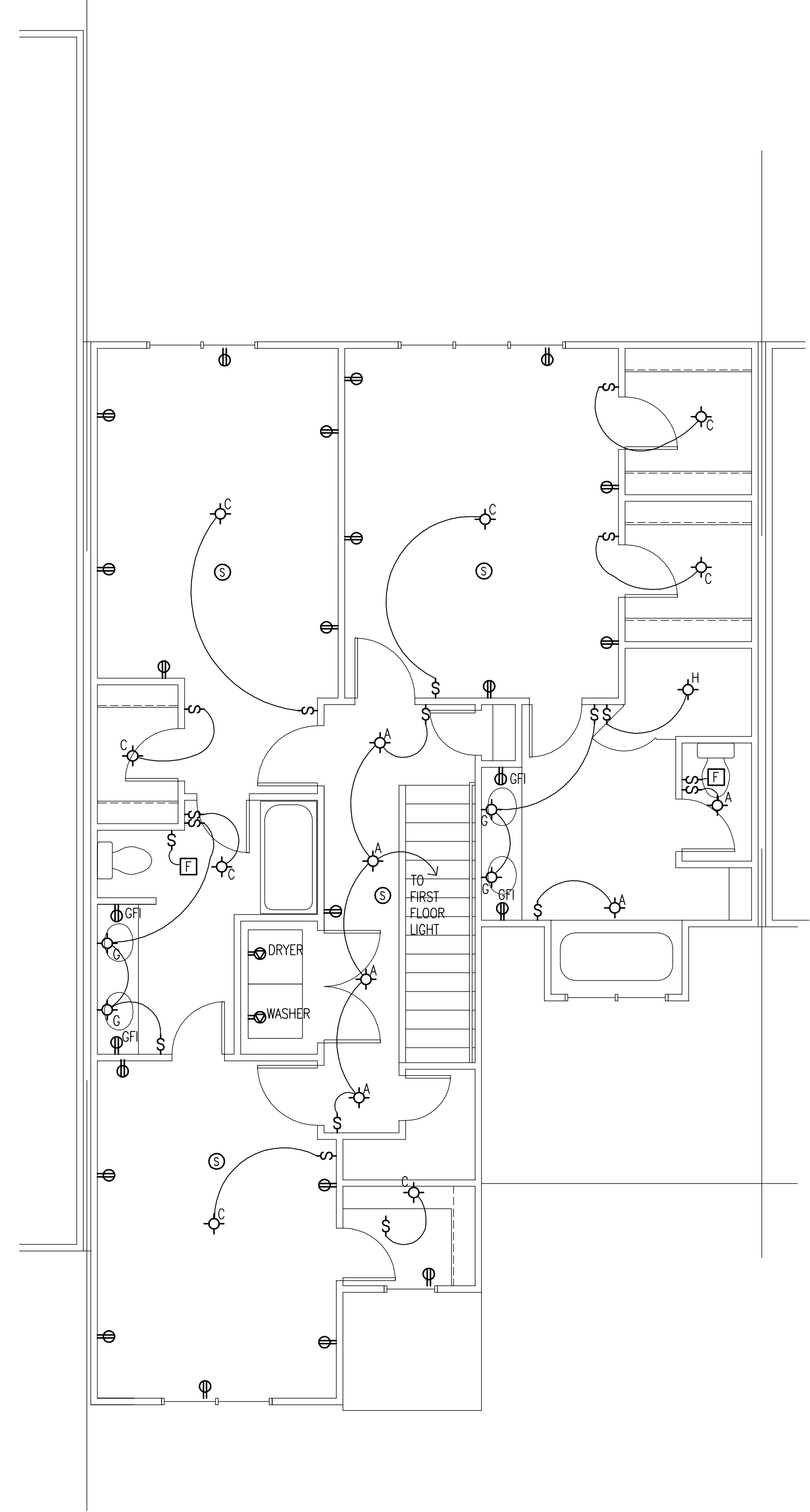
1 SECOND FLOOR ELECTRICAL PLAN plan NORTH A6 SCALE: 1/4"=1'-0"
