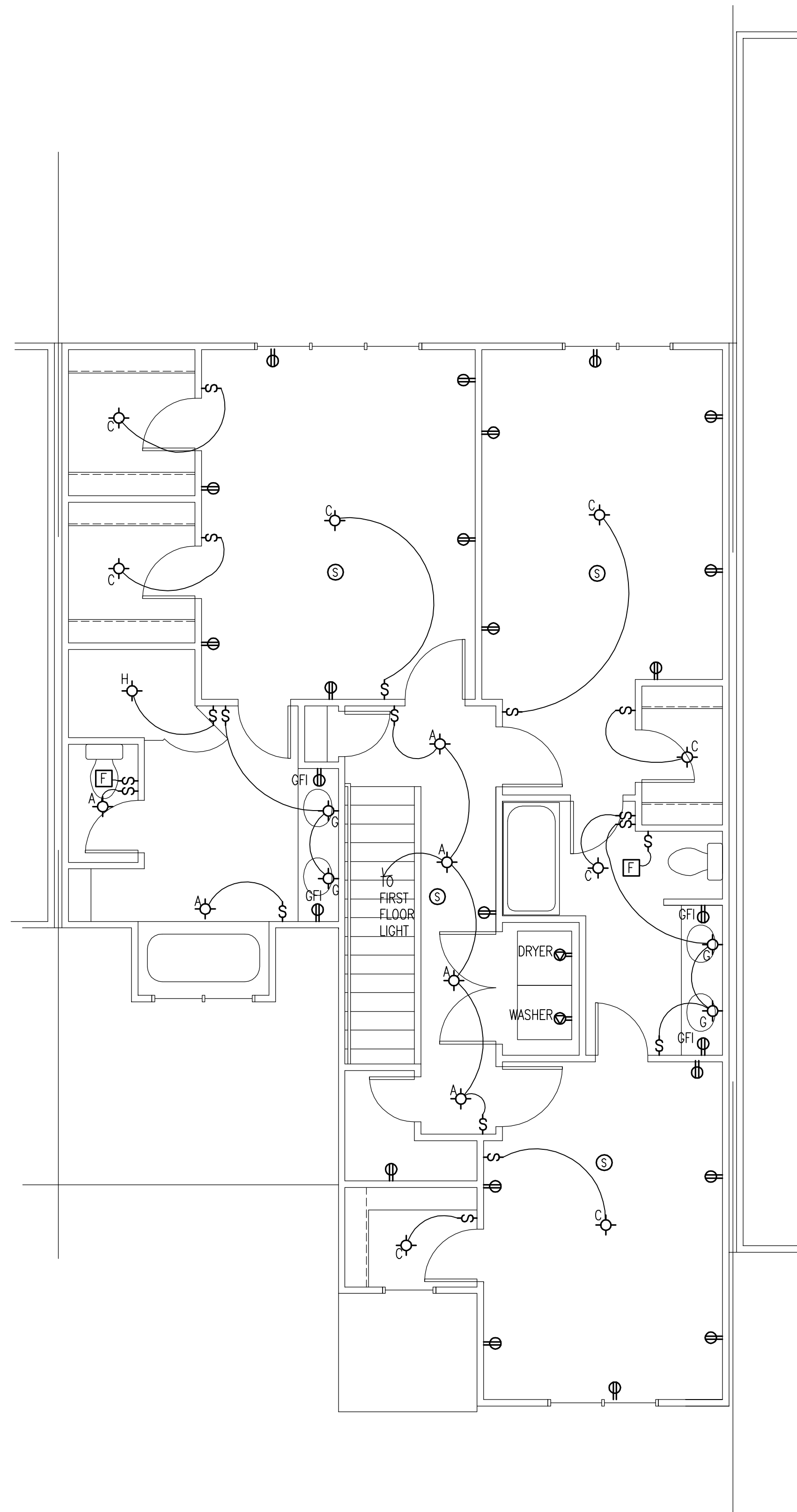
1 SECOND FLOOR ELECTRICAL PLAN plan NORTH A6 SCALE: 1/4"=1'-0"
