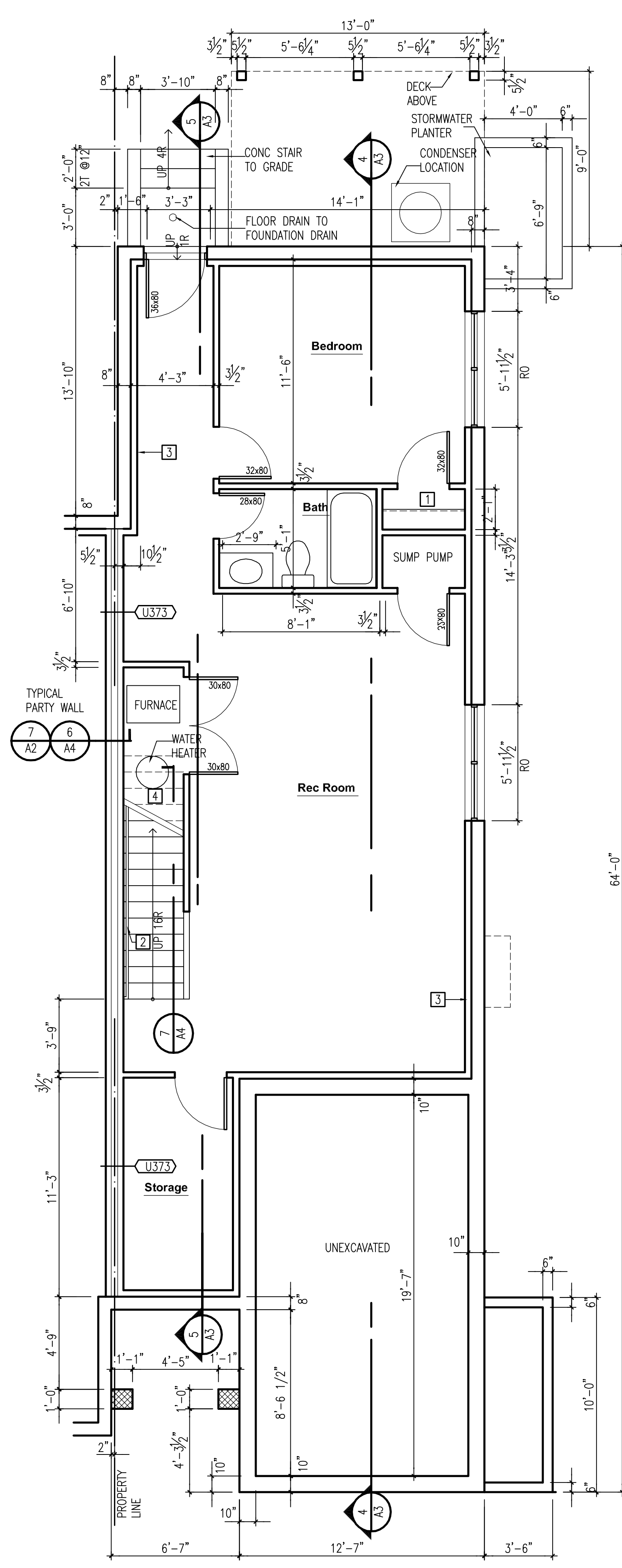
1 BASEMENT FLOOR PLAN plan SCALE: 1/4"=1'-0" NORTH
