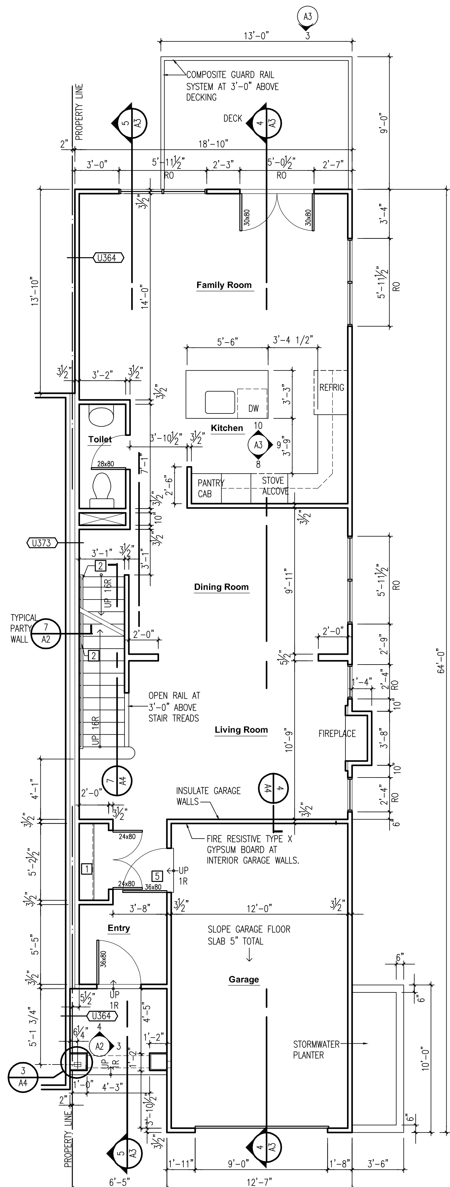
2 FIRST FLOOR PLAN plan SCALE: 1/4"=1'-0" NORTH
