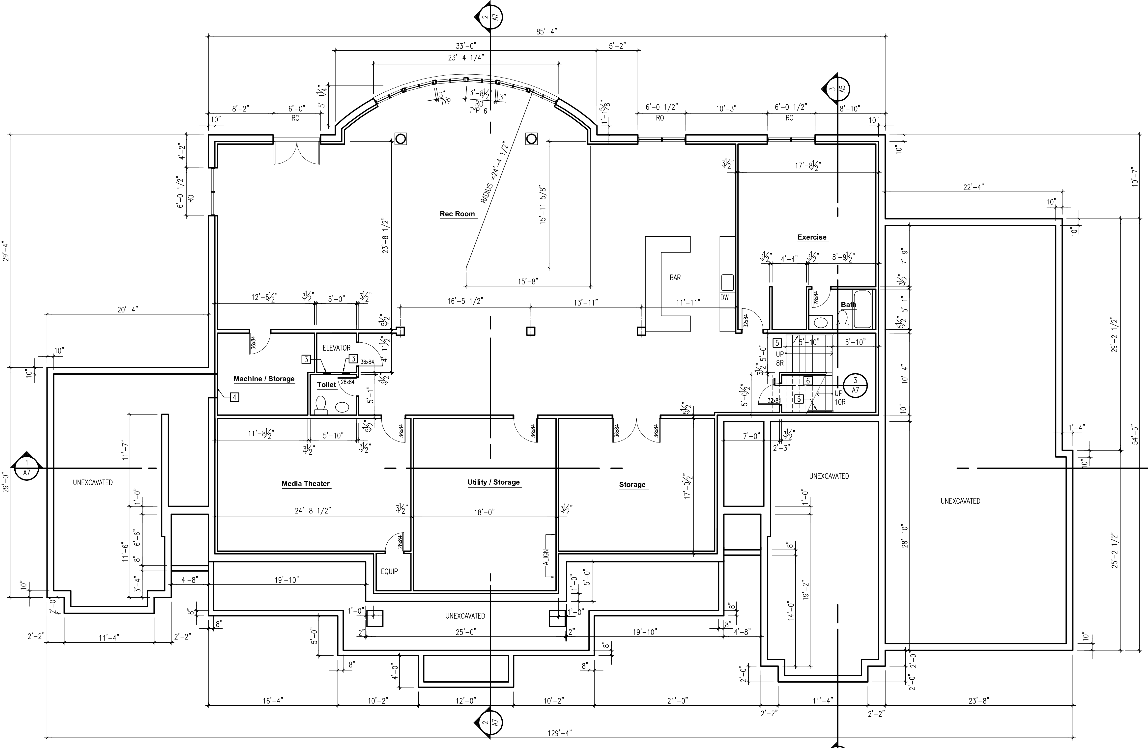
1 A1 BASEMENT PLAN SCALE: 3/16"=1'-0" plan NORTH
