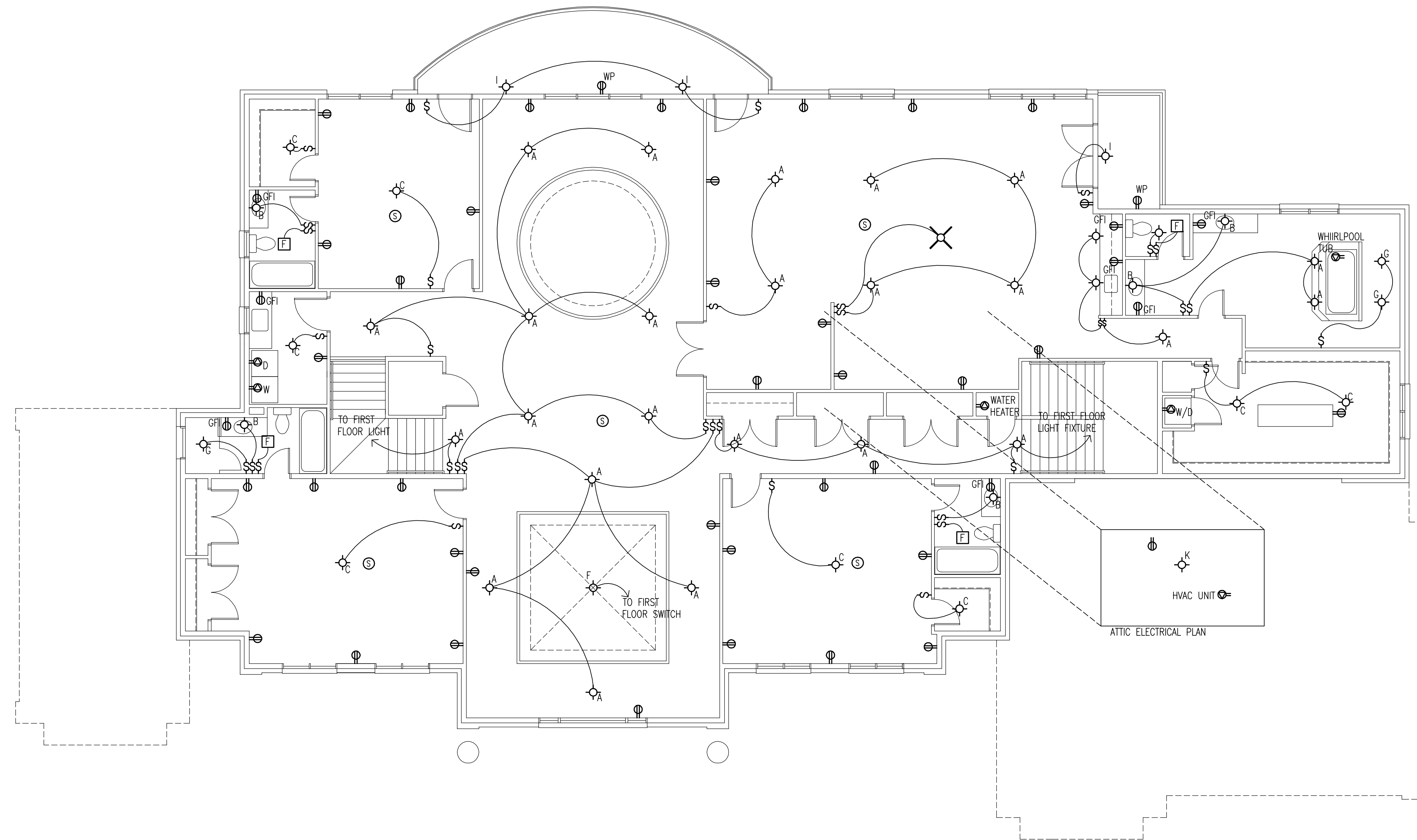
1 SECOND FLOOR ELECTRICAL PLAN A11 SCALE: 1/4"=1'-0" NORTH
