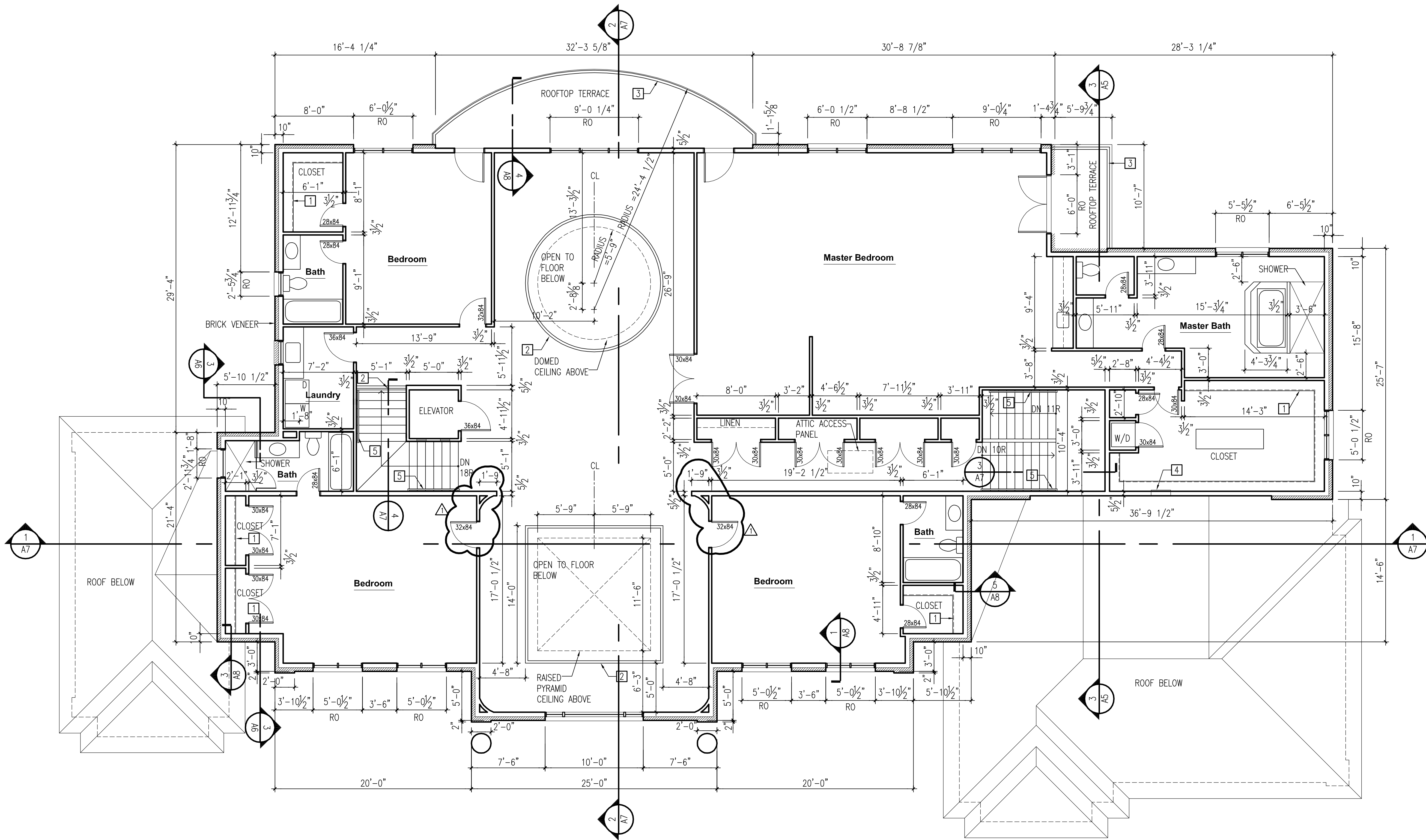
1 SECOND FLOOR PLAN SCALE: 3/16"=1'-0" plan NORTH
